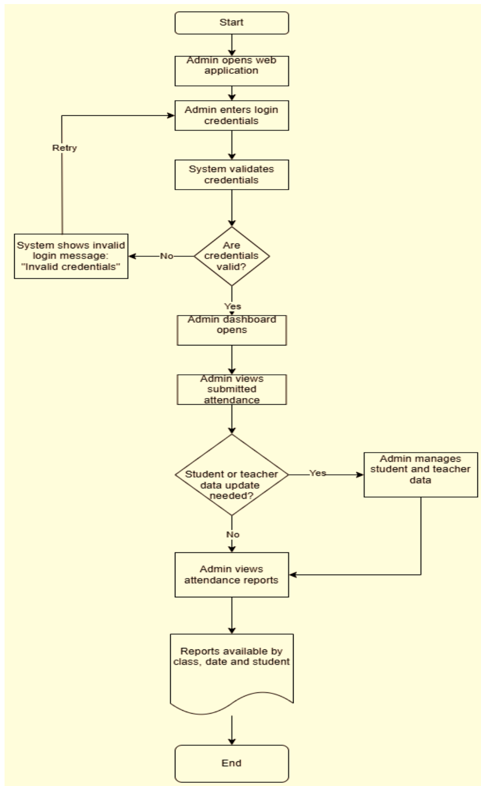
Diagram 2: Admin Attendance Review Flow
