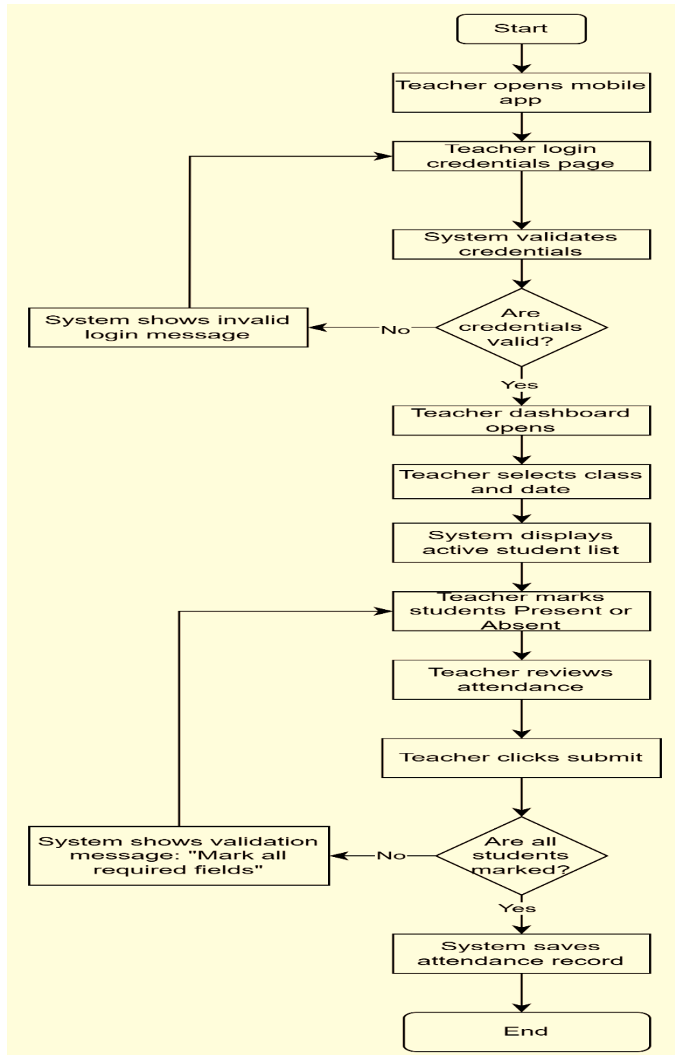
Diagram 1: Teacher Attendance Submission Flow
